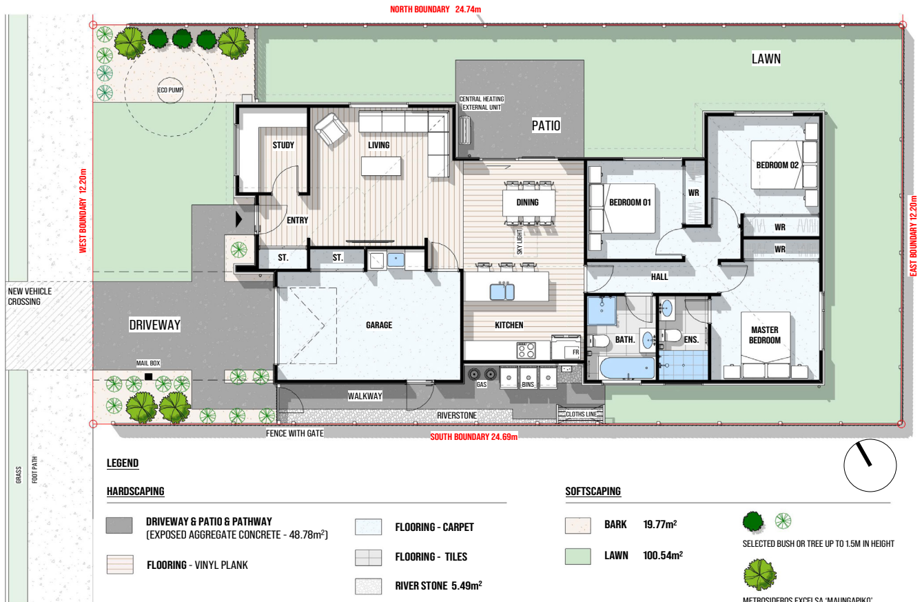
FLOOR PLAN
