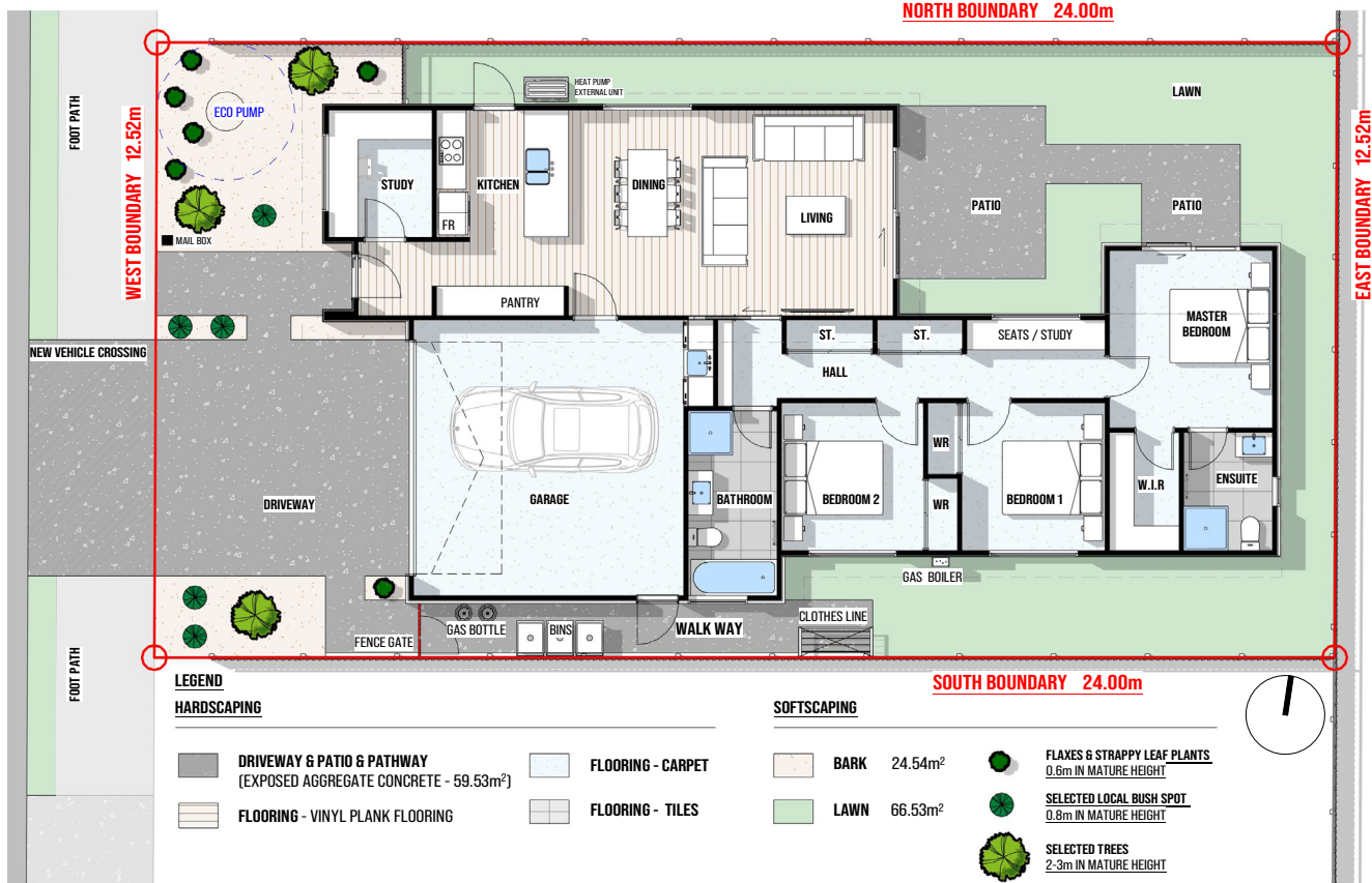
FLOOR PLAN
